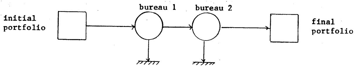
Figure 2: Hierarchy
