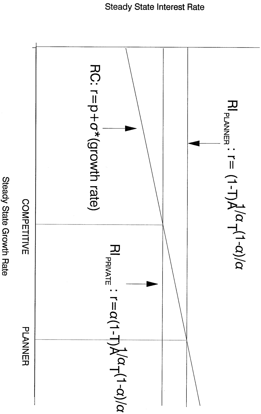
FIGURE 3: BARRO MODEL
