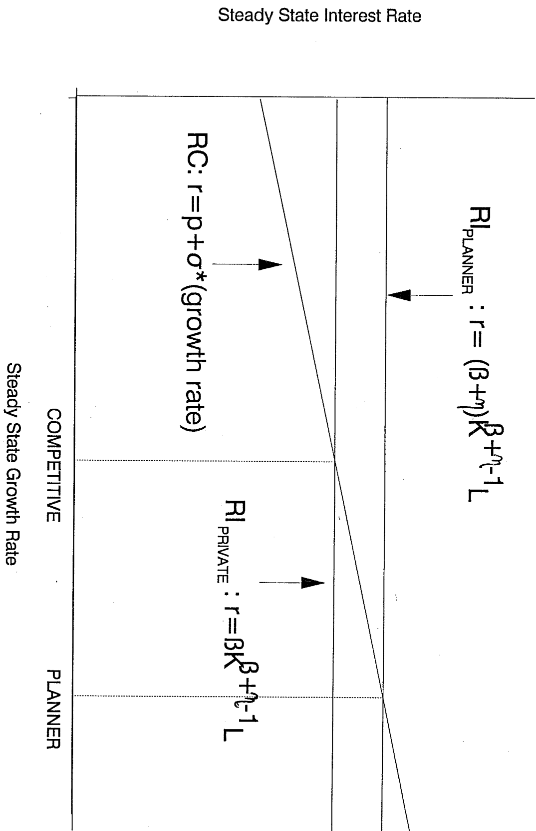
FIGURE 4: ARROW-SHESHINSKI-ROMER MODEL
