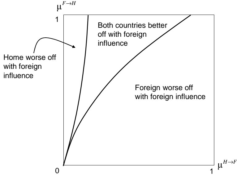
Figure 5: Pareto Gains with Asymmetric Functions
