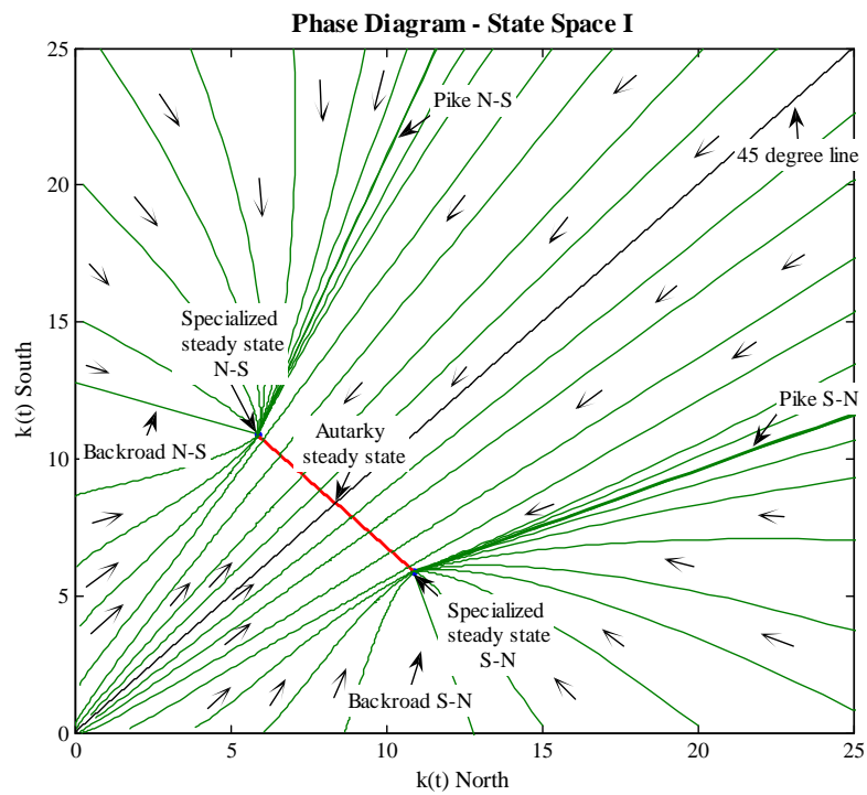
Figure 11: The figure presents the complete phase diagram for State Space I for any initial condition. The arrows indicate the directions of the trajectories. The complete set of steady states are presented including the autarky steady state.
