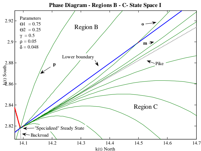
Figure 10: The figure presents sample trajectories in State Space I for the case in which countries leave the FPE set in finite time. Consider a trajectory like "o". Countries start trading with FPE and both countries produce positive amounts of both goods. As they develop we observe that south will find cost advantageous to specialize in the production of the labor intensive good. This happens when countries leave the FPE set in the figure and they move to region C. After that, countries converge to a steady state where south remains specialized (Specialized Steady state in the picture). There is a tendency towards FPE at the steady state. During the transition factor prices were equal initially, then not.
