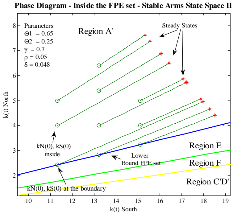
Figure 5: This figure presents several exact trajectories for the case where countries start trading inside the FPE set (region A'). See note in figure 4 for a description of the findings for the case of State Space I.
