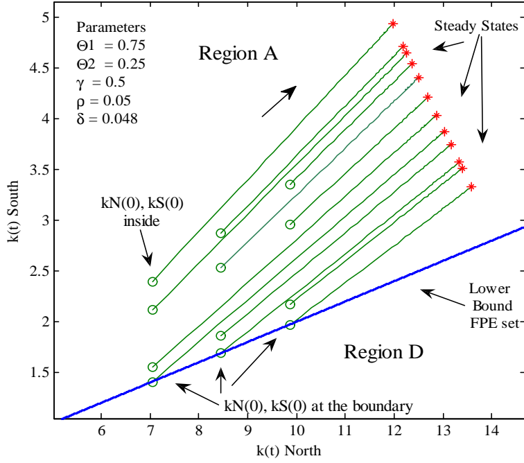
Phase Diagram - Inside the FPE set - Stable Arms State Space I
