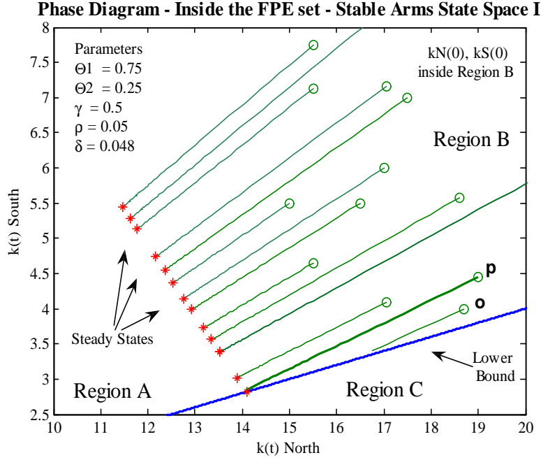
Figure 6: This figure presents several exact trajectories for the case of State Space I and where countries start trading inside the FPE set and above the steady state (region B). Consider any initial condition (circles) above trajectory p . Factor prices equalize and countries produce positive amount of both tradable goods along the transition path. Countries reach a steady state (stars) strictly inside the FPE set. Now consider trajectory p . In this case, countries start trading inside the FPE set but converge to a steady state at the lower boundary of the FPE set. At the boundary, factor prices are equal but south specializes in the production of the labor intensive good. Therefore, during the transition to the steady state, south changes the pattern of specialization from diversified to fully specialized in the production of the good that it has a comparative advantage.
