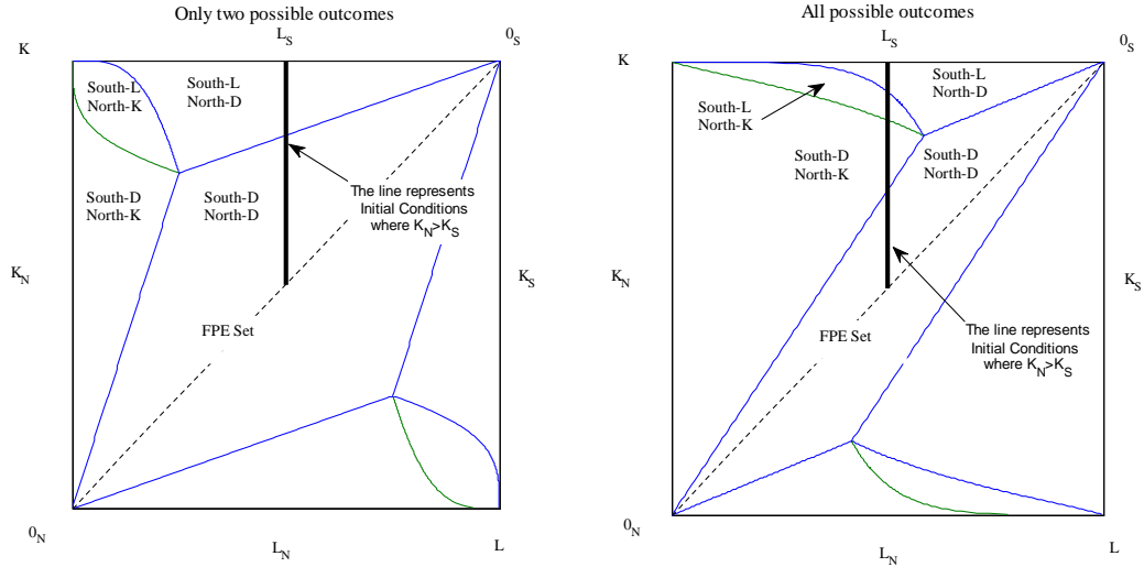
Figure 1: The figure illustrates the possible patterns of specialization, and how they might change according to initial conditions. South - L refers to the case in which South is specialized in the production of the labor intensive good. North - K refers to the case in which North is specialized in the production of the capital intensive good. North - D and South -D refer to the case in which both countries are diversified in production, producing positive amounts of labor and capital intensive goods. The darker line reflects initial conditions where the endowments of capital from North are larger than the endowments of capital from South and labor is equal in both countries. The difference between the figure on the left hand side (LHS) and the right hand side (RHS) are parameter values. Both figures have the same initial conditions over the countries and world endowments. The figure on the LHS shows that there are only two possible outcomes, either both countries are diversified in production or North is diversified and South L-specialized. The RHS figure shows that all possible outcomes are possible.
