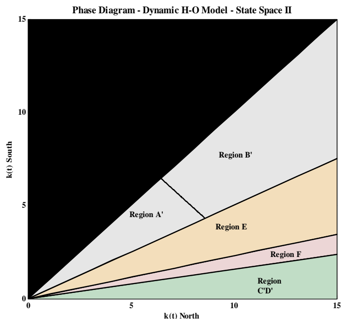
Figure 3: The figure divides the (k^N - k^S) plane into different regions for the case in which k^N(0) > k^S(0) . In regions A' and B' both countries are diversified and factor prices are equalized (FPE) (North-D, South-D). In region E north specializes in the production of the capital intensive good, while south produces both goods (North K-specialized, South-D). Region F corresponds to the full specialization case (North K-specialized, South L-specialized). Region C'D' south is specialized in the production of the labor intensive good and north diversified (North-D, South L-specialized). The upper half part of the picture is not presented because k^N(0) > k^S(0) \Rightarrow k^N(t) > k^S(t) for all t (Proposition 2).
