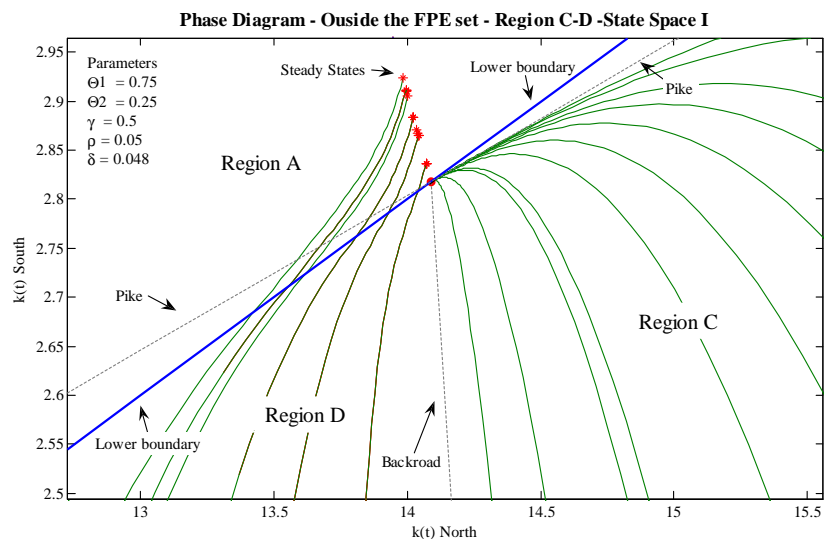
Figure 8: This figure presents sample paths for countries that start trading without FPE. Consider any initial condition in region C. In region C, south specializes in the production of the labor intensive good and north diversifies. Note that north is above its steady state while south is below. The figure shows that during the transition to the steady state south overshoots its long run steady state. It remains specialized during the transition and at the steady state (never leaves region C) During the transition factor prices are not equal and in the long run there is a tendency towards factor price equalization. Note that trajectories that start in C reach the pike before they reach the FPE set. Consider now initial conditions to the left of the backroad (region D). Countries start trading below the steady state. South produces only the labor intensive good, while north diversifies. In finite time south diversifies its production (when the trajectories cross to region A) and there is factor price equalization (they reach the FPE set before they reach the pike).
