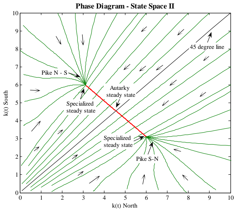
Figure 12: The figure presents the complete phase diagram for State Space II for any initial condition. The arrows indicate the directions of the trajectories. The complete set of steady states are presented including the autarky steady state.
