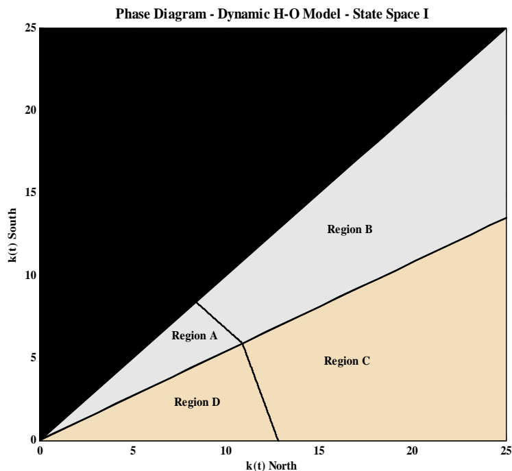
Figure 2: The figure divides the (k^N - k^S) plane into different regions for the case in which k^N(0) > k^S(0) . In regions A and B both countries are diversified and factor prices are equalized (FPE) (North-D, South-D). In regions D and C south is specialized in the production of the labor intensive good and north diversified and there is no FPE (North-D, South L-specialized). The line dividing regions A and B from C and D is the lower bound of the FPE set. The upper half part of the picture is not presented because k^N(0) > k^S(0) \Rightarrow k^N(t) > k^S(t) for all t (Proposition 2).
