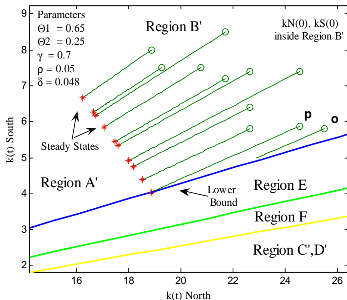
Figure 7: This figure presents several exact trajectories for State Space II and the case where countries start trading inside the FPE set and above the steady state (region B'). Consider any initial condition (circles) above trajectory p . Factor prices equalize and countries produce positive amount of both tradable goods along the transition path. Countries reach a steady state (stars) strictly inside the FPE set. Now consider trajectory p . In this case, countries start trading inside the FPE set but converge to a steady state at the lower boundary of the FPE set. At the boundary, factor prices are equal but north specializes in the production of the capital intensive good. Therefore, during the transition to the steady state, north changes the pattern of specialization from diversified to fully specialized.
