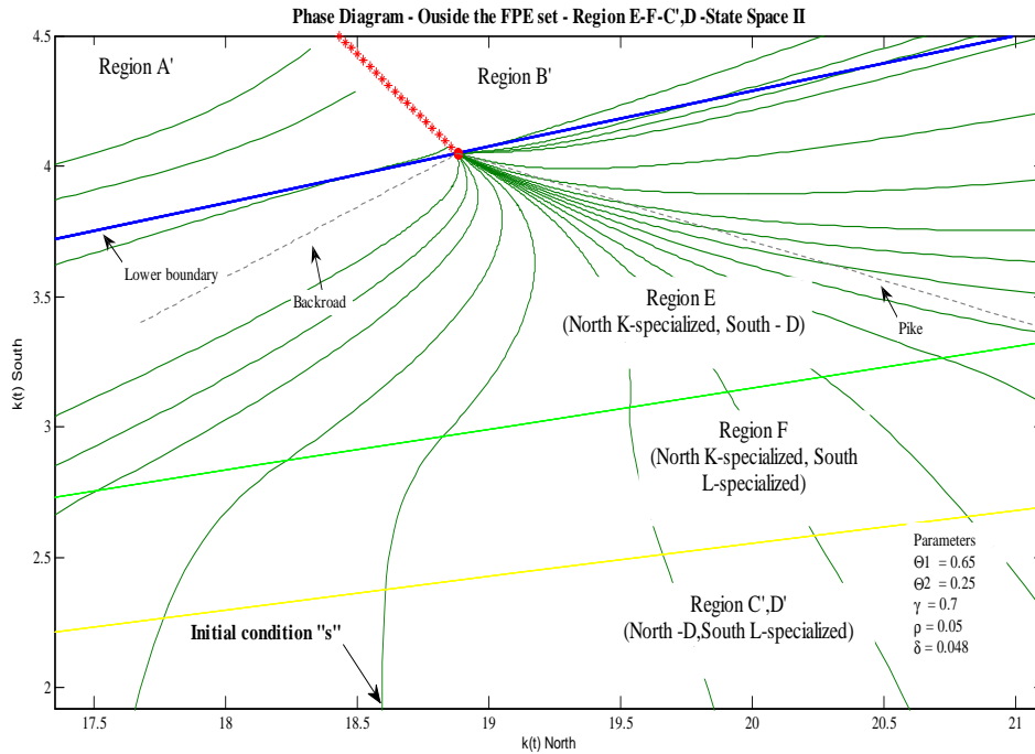
Figure 9: The figure presents sample trajectories for State Space II for the cases where countries start trading outside the FPE set and at least one country is fully specialized. As we can see, there are no monotonic changes in the pattern of specialization. Consider initial condition "s" in the figure where south is far away from the steady state and north is close to its steady state. Countries start in region C'D' where south specializes in the production of the labor intensive good and north diversifies. As countries develop, south accumulates capital faster than in north (note that the slope of the trajectory is very steep). Eventually countries reach region F where both are specialized. Note that during this transition south is the country that accumulated more capital. As they develop, countries eventually reach region E, where north remains specialized and south diversifies. Note that when this happens, north overshoots its long run steady state converging to it from above. It is also important to note in this picture how the slopes of the pike and the backroad changed compared to the case of State Space I.
