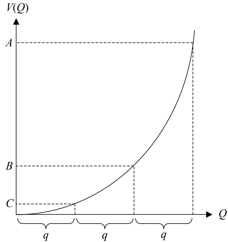
Panel B: Convex Surplus Function
