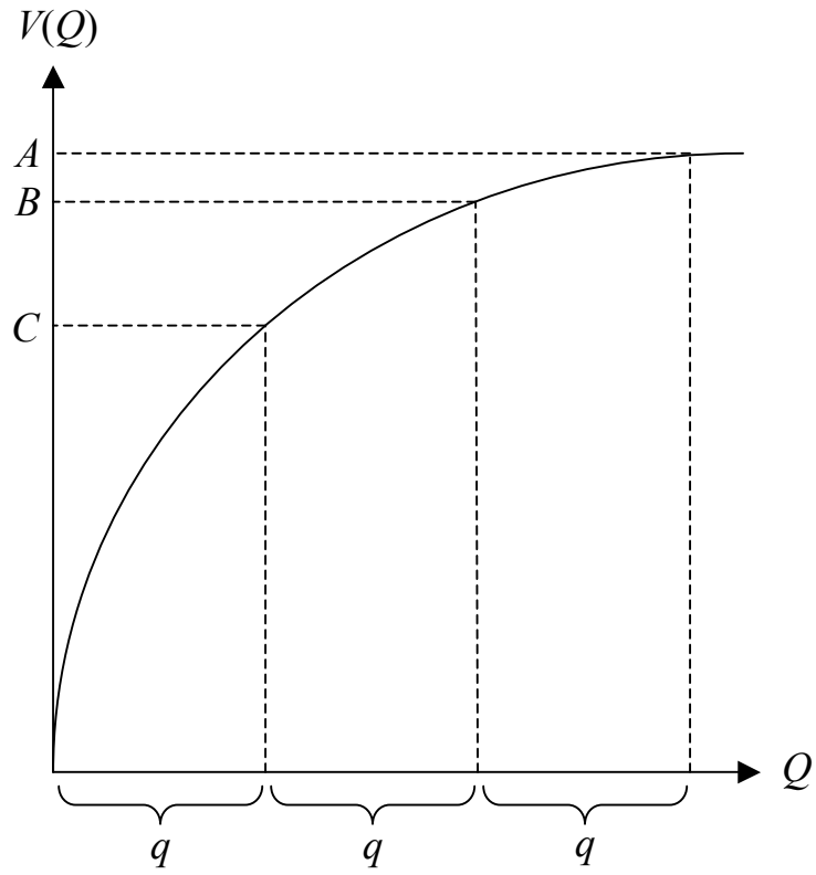
Panel A: Concave Surplus Function
