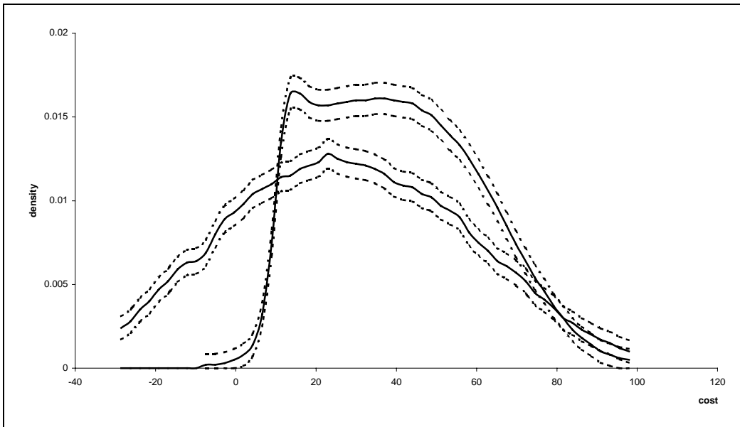
Figure 6d: Probability density functions of total cost
