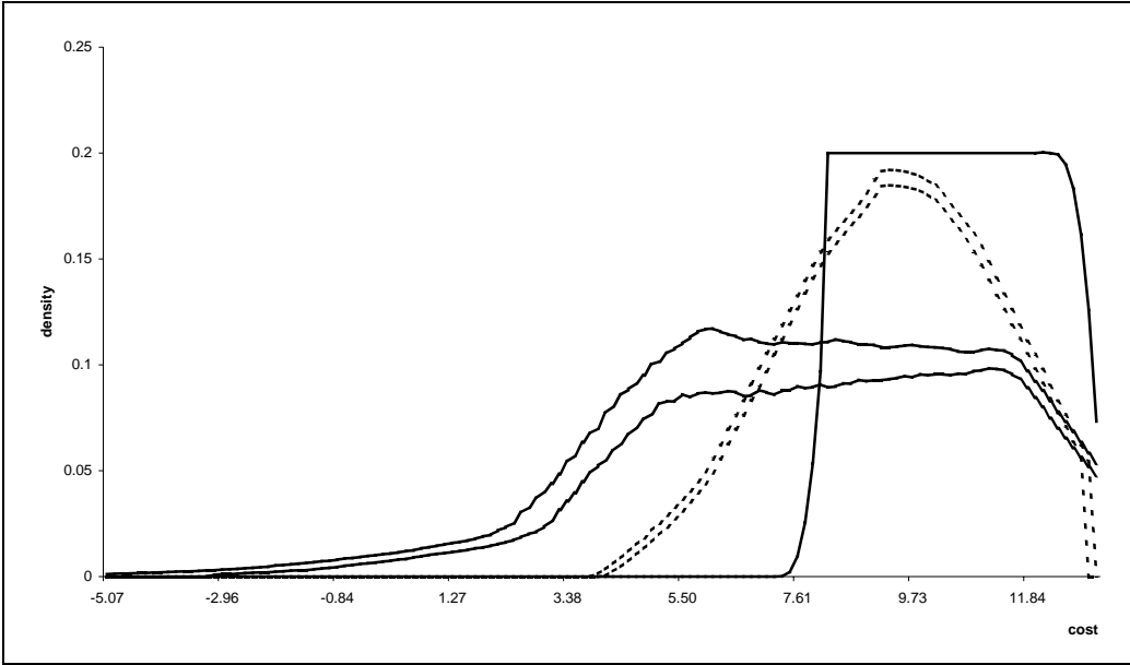
Figure 7b: Probability density function of total cost, s=5 , (5% and 95% pointwise quantiles of estimators)
