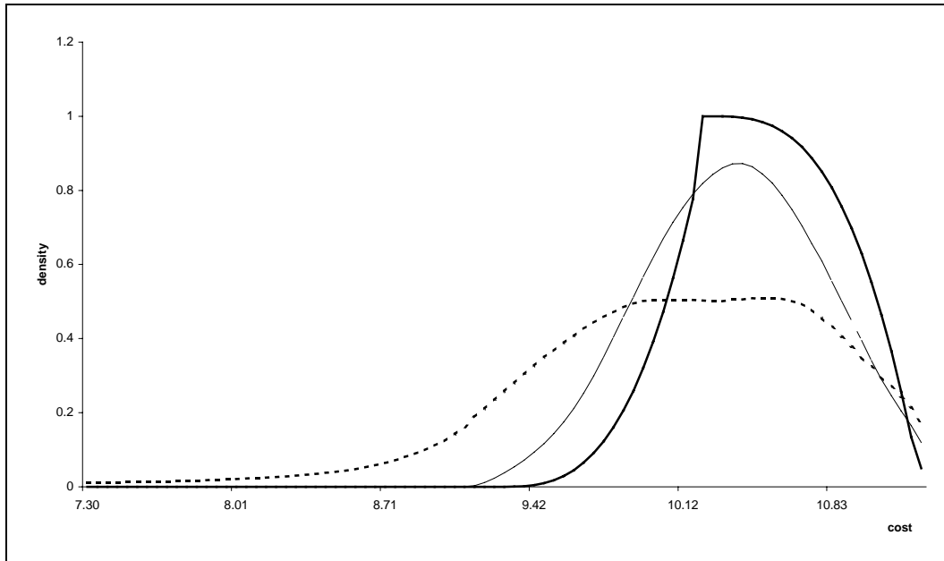
Figure 6b: Probability density function of total cost, s = 1
