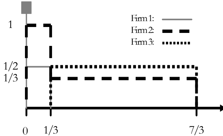
Equilibrium in the Multiplication Game
