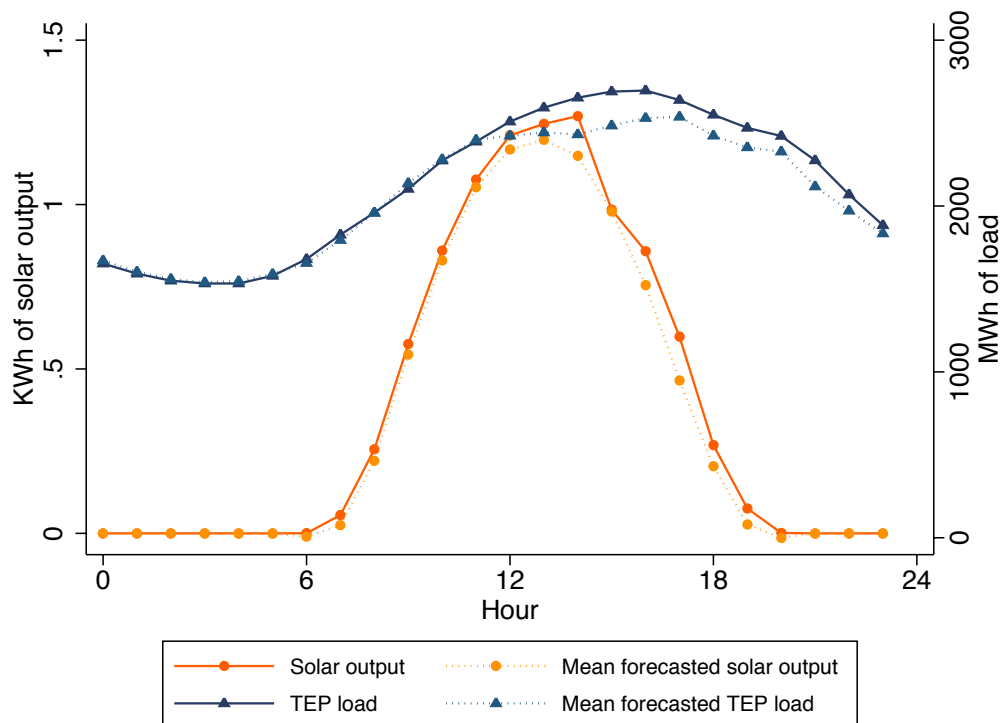
Figure 1: Predicted and actual Tucson load and solar output, Jul. 15, 2008
