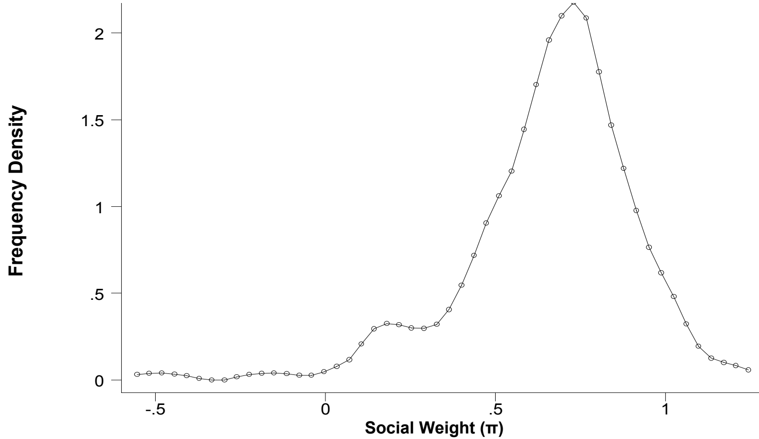
Figure 9: Kernel Density Estimates of Social Weight ( \pi )
