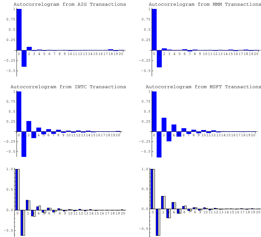
Fig. 4. Top and middle panels: Log-return autocorrelations from transactions for American International Group, Inc. (AIG), 3M Co. (MMM), Intel (INTC) and Microsoft (MSFT), last ten trading days in April 2004. Bottom panel: log-return autocorrelation from the same transactions for Intel and Microsoft, superimposed with the autocorrelation fitted from the basic i.i.d. plus AR(1) model for the noise.
