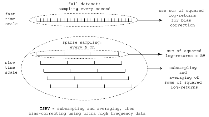
Fig. 3. This figure describes the construction of the TSRV estimator.
