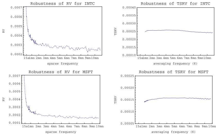
Fig. 8. Comparison of the RV and TSRV estimators for Intel and Microsoft, averaged over the last ten trading days of April 2004. The left panels demonstrate the dependence of RV as a function of the sparse sampling interval, while the right panels study the robustness of TSRV with respect to the choice of the averaging frequency as represented by the number of subgrids K . The estimators were calculated from transaction data.
