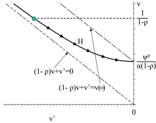
Figure 1: The function H
