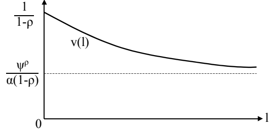
Figure 2 : The function v(l)
