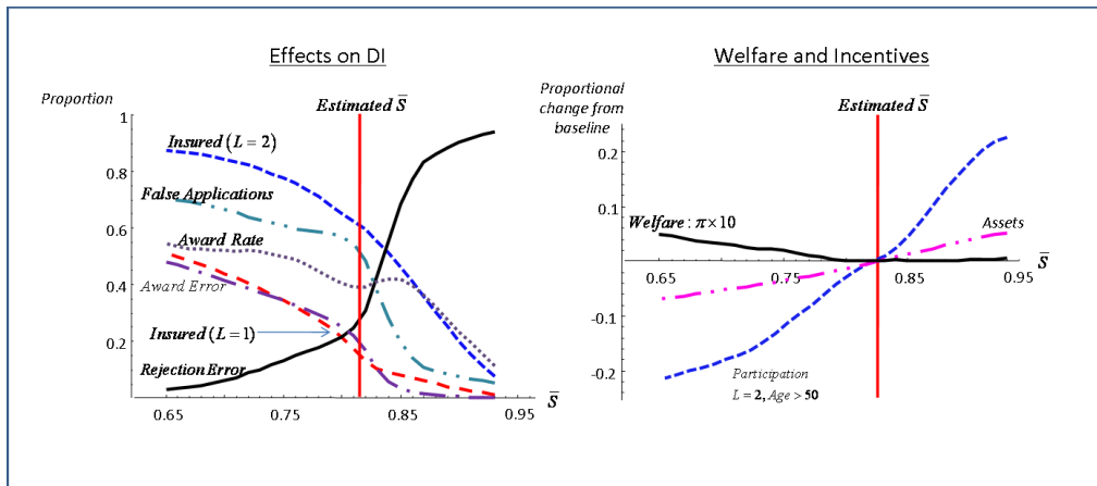
Figure 3: Changing strictness
