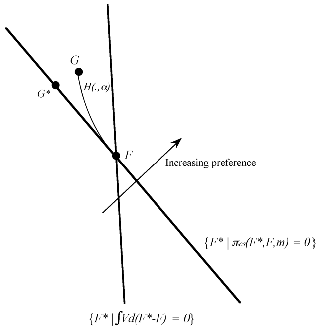
Figure 1. Why the percentage error from using ECS is unbounded: for any sequence G_n along the path H , \pi_{cs} tends to 0 faster than \pi - \pi_{cs} .
