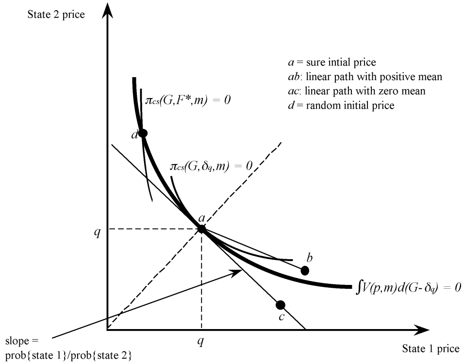
Figure 2: Illustration of Theorem 3
