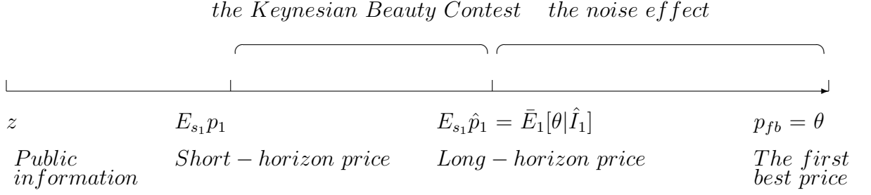
Figure 2 : The Keynesian Beauty Contest and Noise Effect
