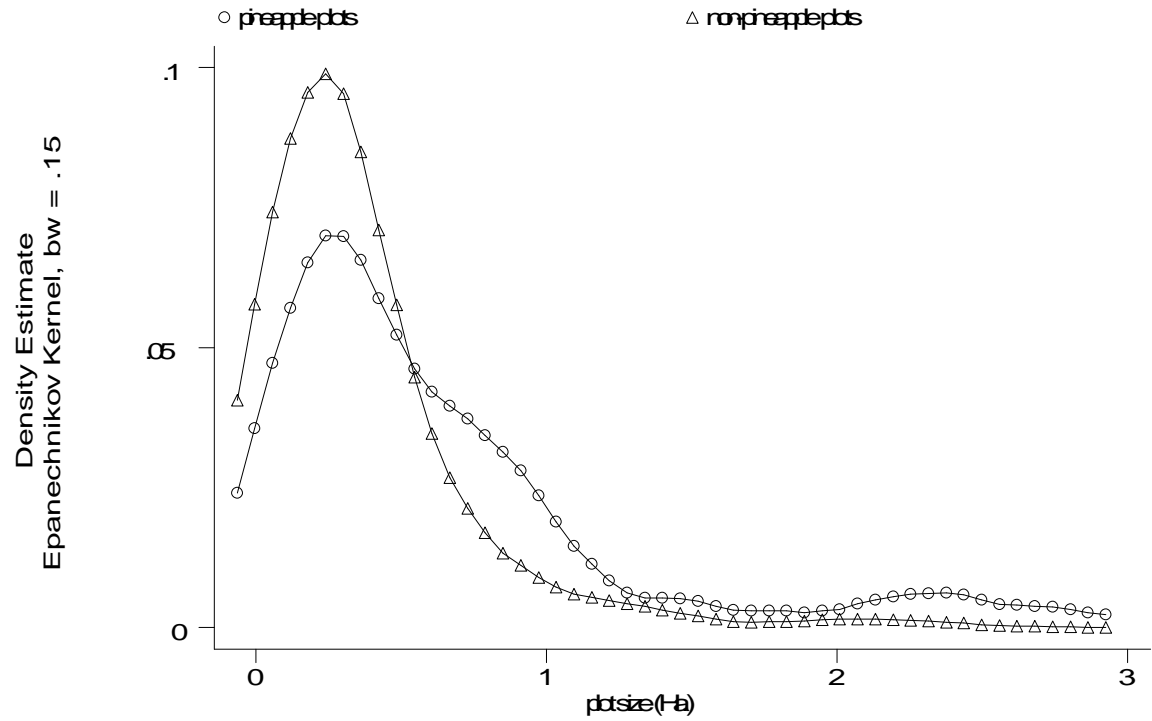
Figure 5: Density of Ptsizes
