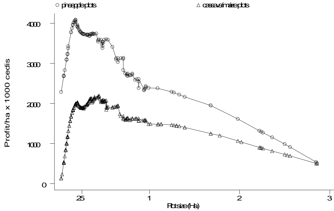
Figure 6: Lowess Estimates of E(\text{profit}/\text{ha} | \text{plot size}) , bw=0.8
