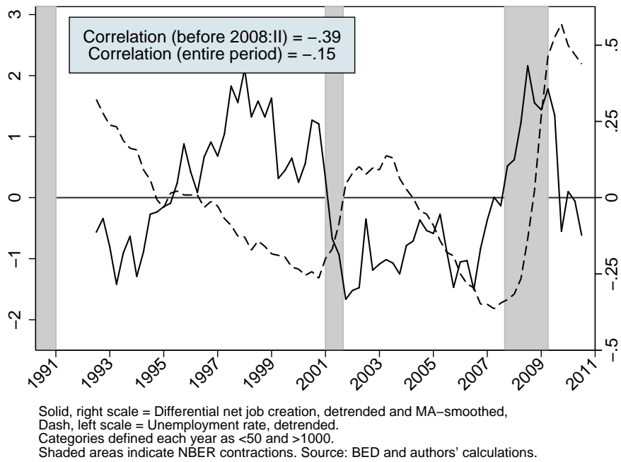
Fig. 6: Differential growth
