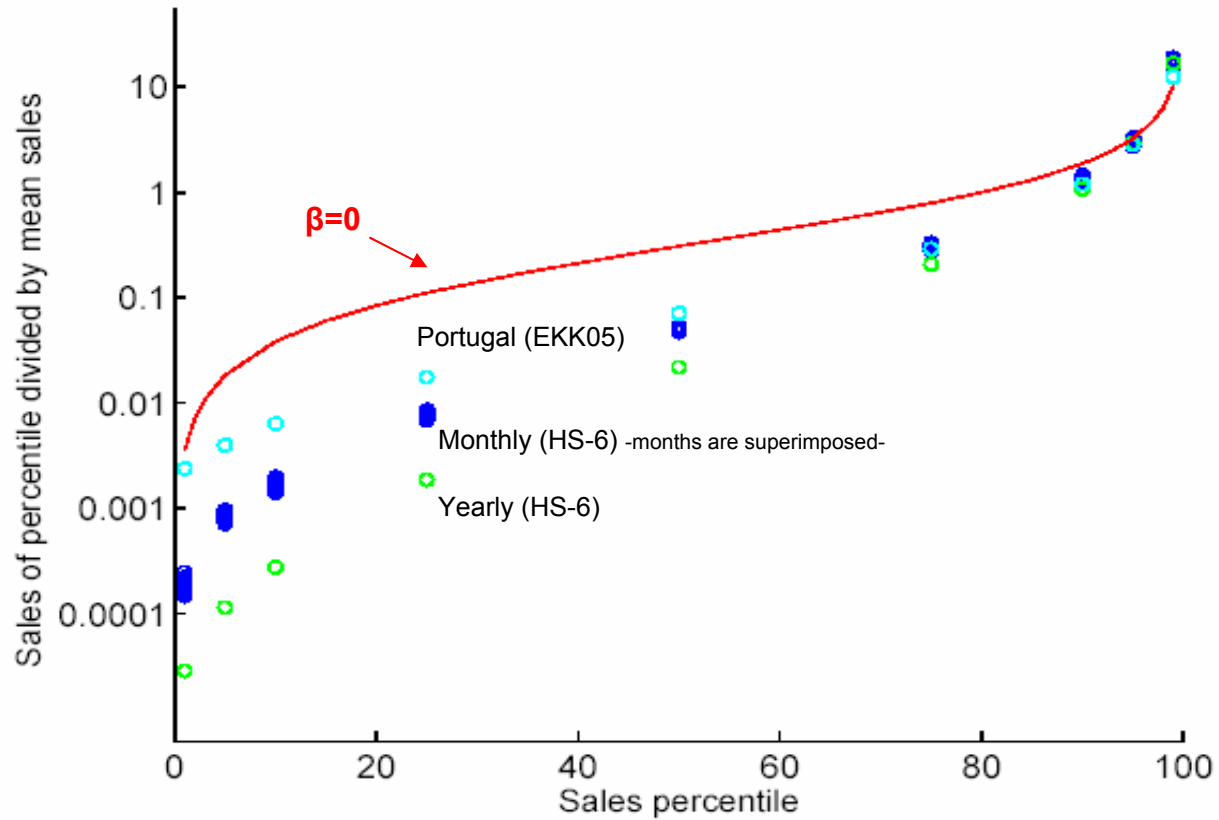
Distribution of sales of US imports from Mex: montly (bl) & yearly (gr) HS-6 data
